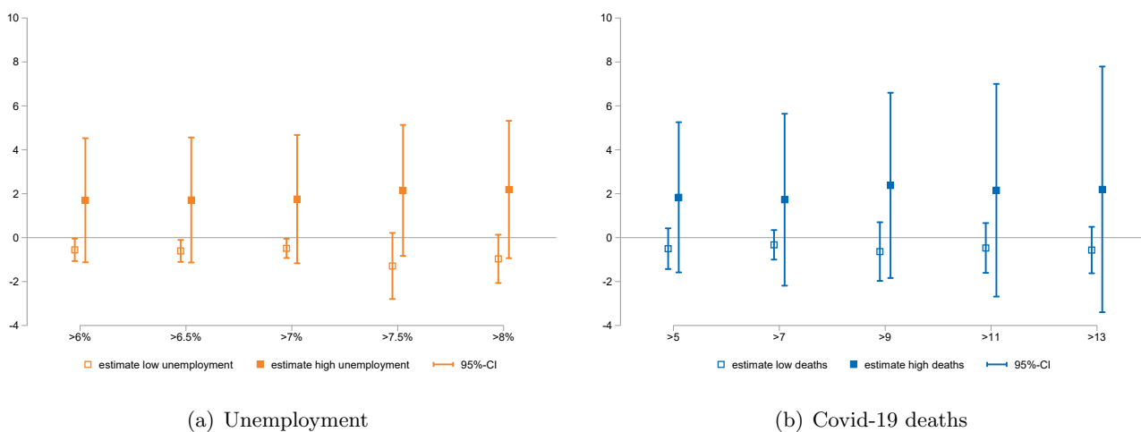
Figure B.3: Robustness: Effect of BAD ECON on social unrest for different thresholds of unemployment rate and COVID-19 deaths
