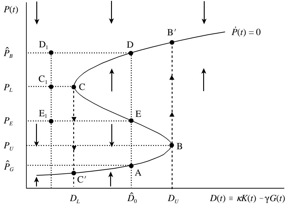
Figure 1: Ecological dynamics
