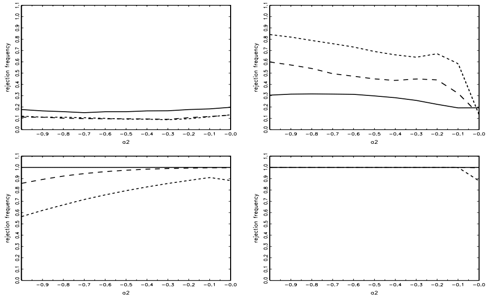
Figure 11: Empirical rejection frequency of hypothesis H_{0+} (left panels) and H_{0-} (right panels) at nominal 10% significance level. Data generation process is \Delta_4 x_t = a_2 x_{t-1}^{(2)} + \varepsilon_t with N(0,1) errors \varepsilon_t . Top panels for RURS-fb test and bottom panels for HEGY test. Solid curve for 100 observations, dashes for 300, and short dashes for 500 observations. 20000 replications.
