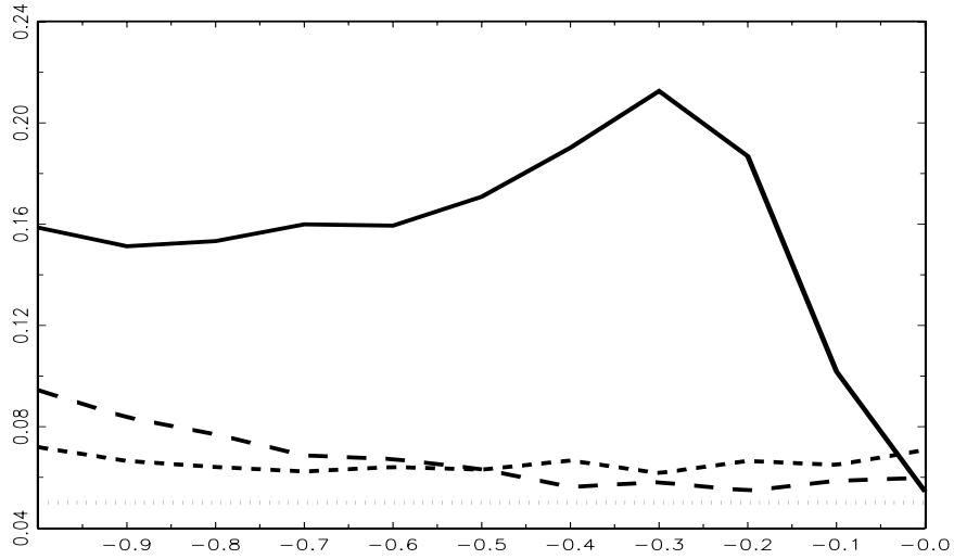
Figure 7: Empirical rejection frequency of unit-root null hypotheses using RURS-fb tests for 200 observations at nominal 5% significance level. Solid curve for \omega = 0 , long dashes for \omega = \pi , and short dashes for \omega = \pi/2 . Generating model is \Delta_4 x_t = a_1 x_{t-1}^{(1)} + \varepsilon_t with N(0,1) errors \varepsilon_t , a_1 on the abscissa axis, 20,000 replications.
