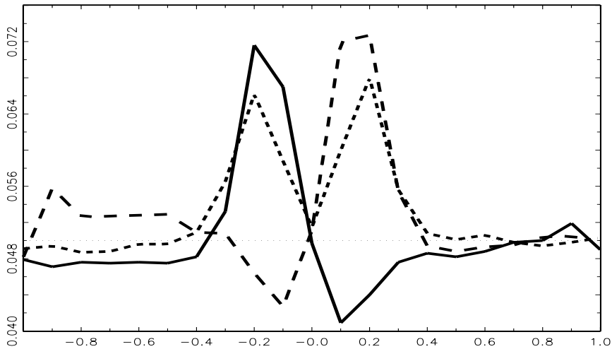
Figure 5: Empirical rejection frequency of unit-root null hypotheses using HEGY t - and F -tests for 200 observations at nominal 5% significance level. Solid curve for t_1 , long dashes for t_2 , and short dashes for F_{34} . Generating model is \Delta_4 y_t = \phi \Delta_4 y_{t-1} + \varepsilon_t with N(0,1) errors \varepsilon_t , \phi on the abscissa axis, 10000 replications.
