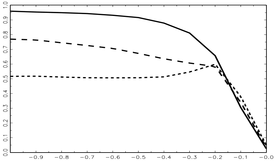
Figure 9: Empirical rejection frequency of unit-root null hypotheses at \omega = \pi using RURS-fb tests for 500 observations at nominal 5% significance level. Upper bound for augmentation varies. Solid curve for the case with no augmentation, dashes for N = n^{1/4} , and short dashes for N = 2n^{1/3} . Generating model is \Delta_4 x_t = a_2 x_{t-1}^{(2)} + \varepsilon_t with N(0,1) errors \varepsilon_t , a_2 on the abscissa axis, 20000 replications.
