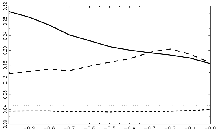
Figure 10: Empirical rejection frequency of unit-root null hypotheses using RURS-fb tests for 200 observations at nominal 5% significance level. Solid curve for \omega = 0 , long dashes for \omega = \pi , and short dashes for \omega = \pi/2 . Generating model is the logit transformation of x for \Delta_4 x_t = a_2 x_{t-1}^{(2)} + \varepsilon_t with N(0,1) errors \varepsilon_t . a_2 on the abscissa axis, 20000 replications.
