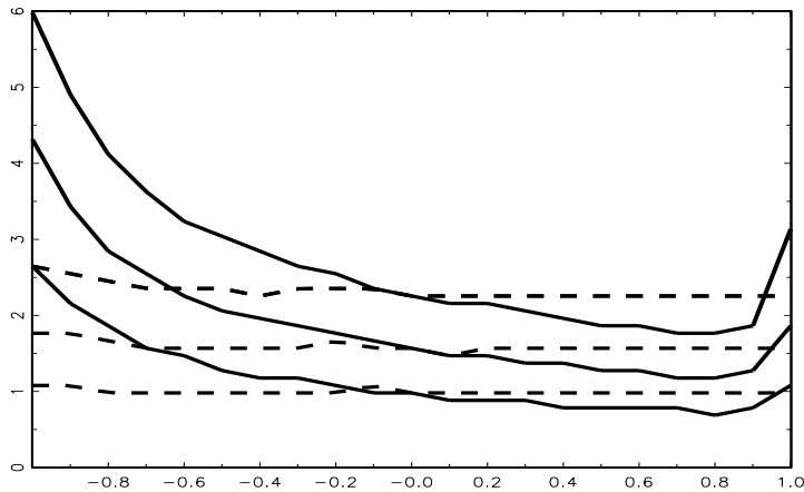
Figure 1: 10%, 50%, and 90% quantiles for the uncorrected (solid) and for the augmentation-corrected (dashed) RURS statistic J_2^{(n)} if it is calculated from trajectories of length n = 100 from the data-generation process \Delta_4 x_t = \phi \Delta_4 x_{t-1} + \varepsilon_t and \phi is varied over the interval [-1, 1] . \phi values on the abscissa.
