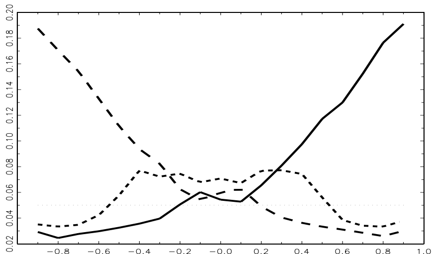
Figure 6: Empirical rejection frequency of unit-root null hypotheses using RURS-fb tests for 200 observations at nominal 5% significance level. Solid curve for \omega = 0 , long dashes for \omega = \pi , and short dashes for \omega = \pi/2 . Generating model is \Delta_4 y_t = \phi \Delta_4 y_{t-1} + \varepsilon_t with N(0,1) errors \varepsilon_t , \phi on the abscissa axis, 20,000 replications.
