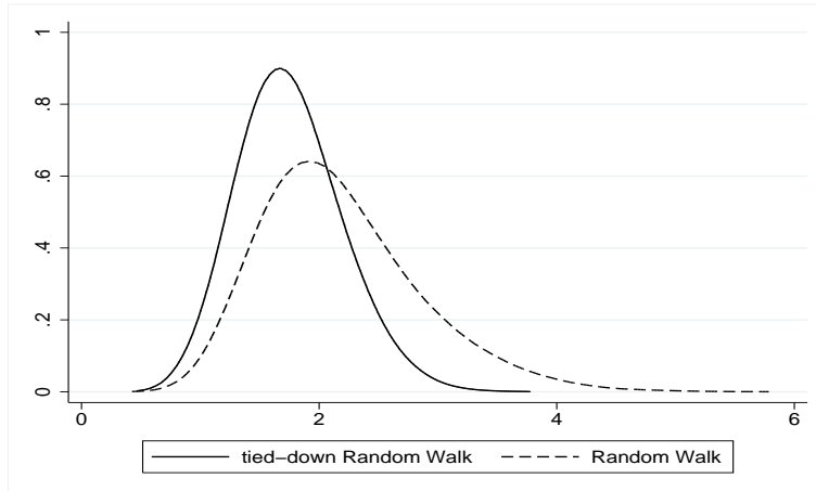
Figure 3: Empirical densities of the RUR statistic for 500 observations. Random walk and drift-adjusted random walk, 20000 replications, Epanechnikov kernel estimation.
