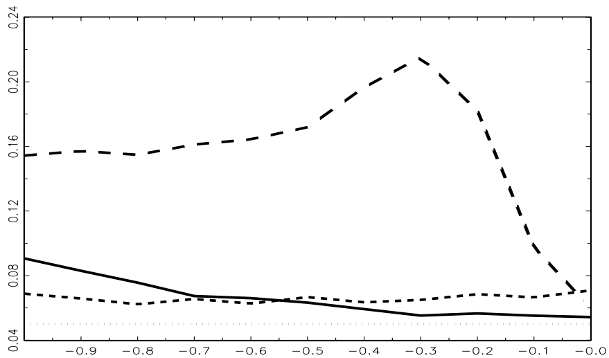
Figure 8: Empirical rejection frequency of unit-root null hypotheses using RURS-fb tests for 200 observations at nominal 5% significance level. Solid curve for \omega = 0 , long dashes for \omega = \pi , and short dashes for \omega = \pi/2 . Generating model is \Delta_4 x_t = a_2 x_{t-1}^{(2)} + \varepsilon_t with N(0,1) errors \varepsilon_t , a_2 on the abscissa axis, 20,000 replications.
