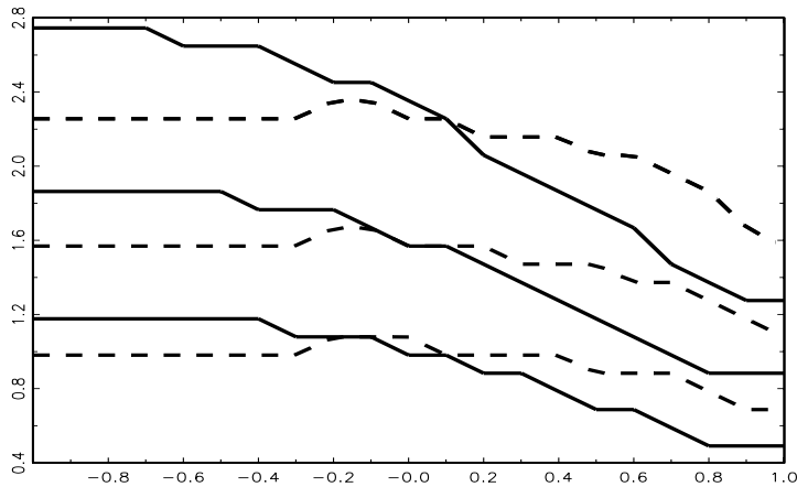
Figure 2: 10%, 50%, and 90% quantiles for the uncorrected (solid) and for the augmentation-corrected (dashed) RURS statistic J_2^{(n)} if it is calculated from trajectories of length n = 100 from the data-generation process \Delta_4 x_t = \varepsilon_t + \theta \varepsilon_{t-1} and \theta is varied over the interval [-1, 1] . \theta values on the abscissa.
