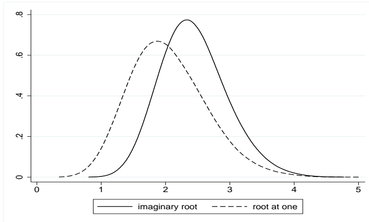
Figure 4: Empirical densities of the RURS statistic for 500 observations. Seasonal random walk, 20000 replications, Epanechnikov kernel estimation.
