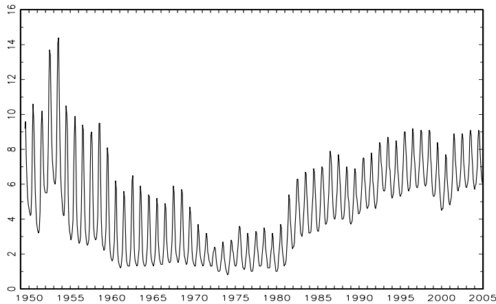
Figure 13: Austrian unemployment rate, 1950:1–2005:12, monthly observations.
