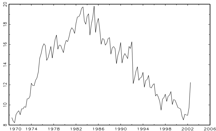
Figure 12: Belgian barley prices, 1971:1–2003:1, quarterly observations.
