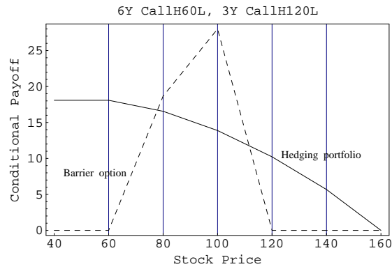
Figure 3: Static hedging strategies allowing liquidation. Conditional values at maturity of the regular options potentially available for hedging (upper panel), of the barrier option and of the hedging portfolio when the short-term option is excluded (middle panel), and when the long-term option with the highest strike is excluded (lower panel).
